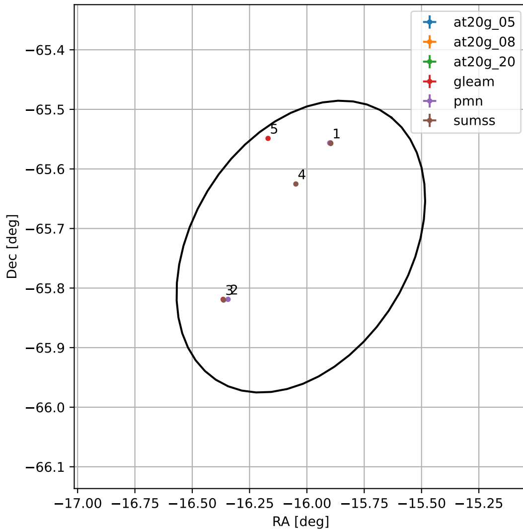
4FGL J2255.8-6543
