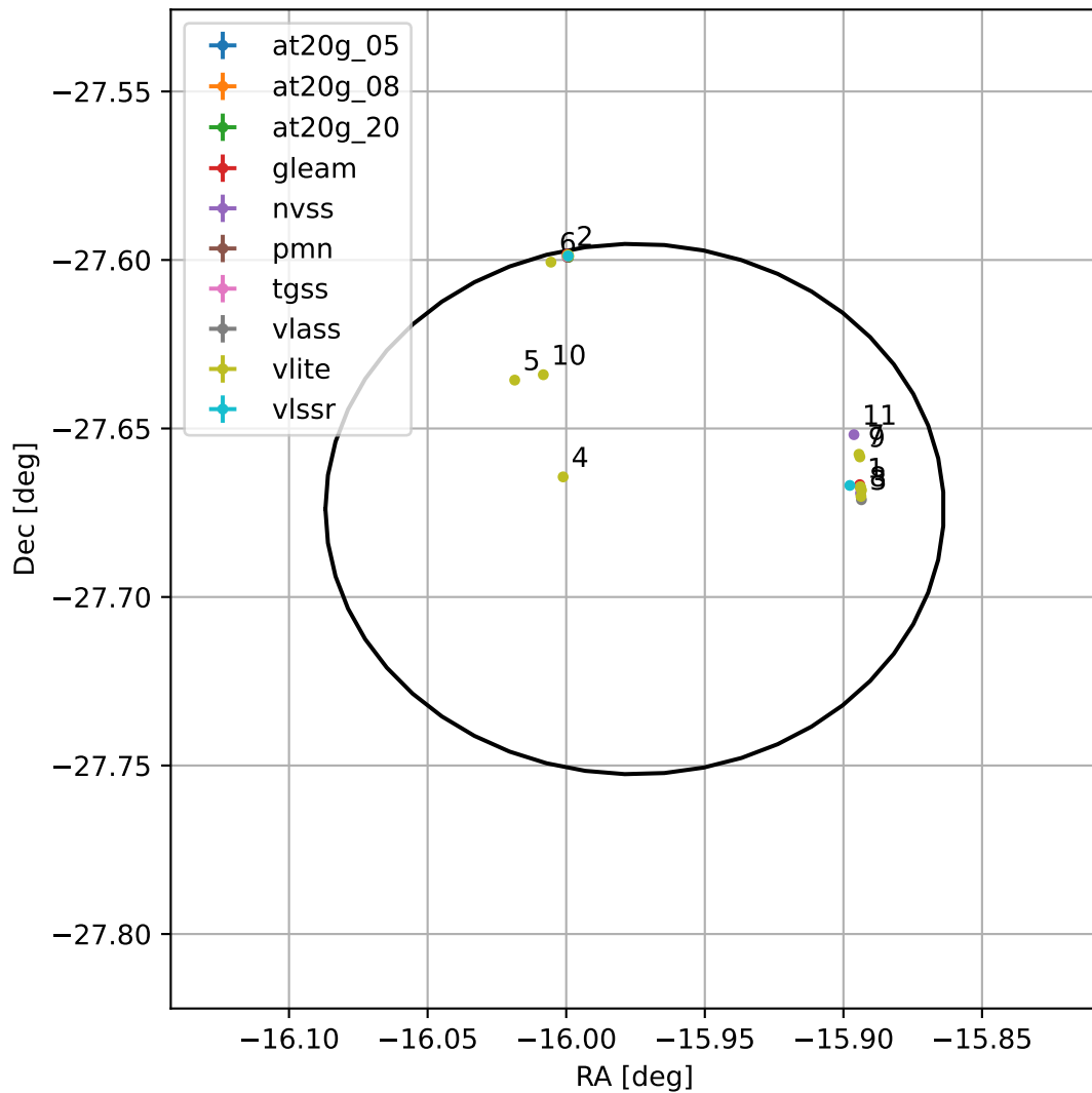
4FGL J2256.0-2740
