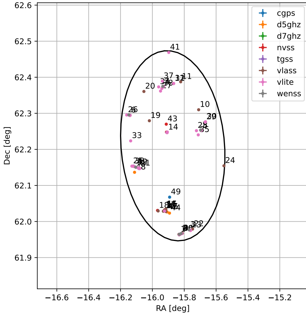
4FGL J2256.5+6212
