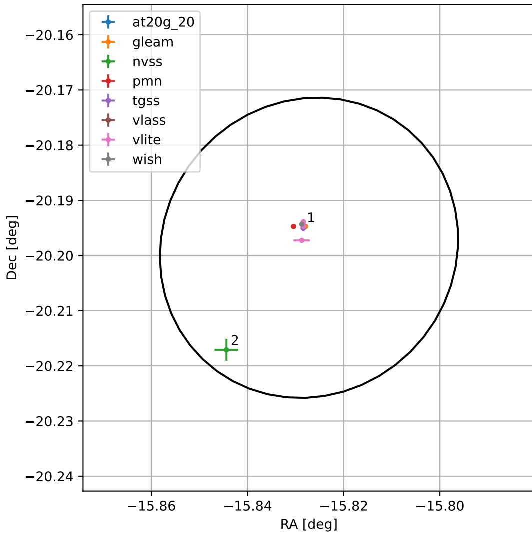
4FGL J2256.6-2011
