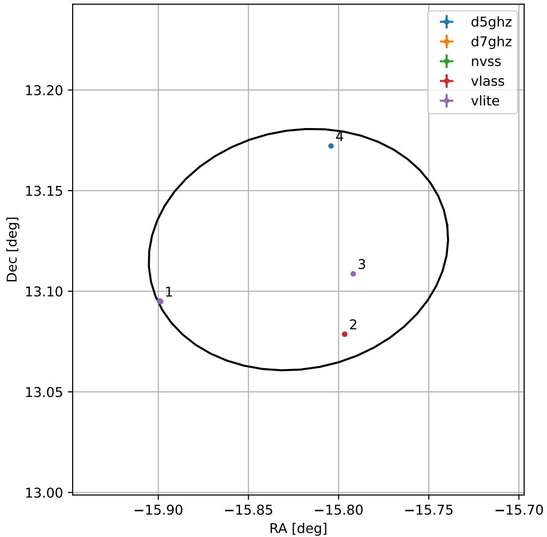
4FGL J2256.7+1307
