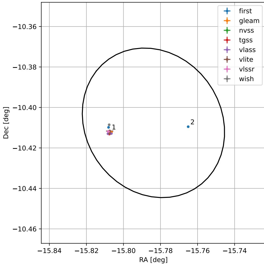
4FGL J2256.8-1024
