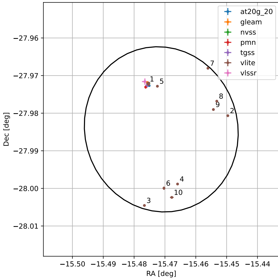
4FGL J2258.1-2759
