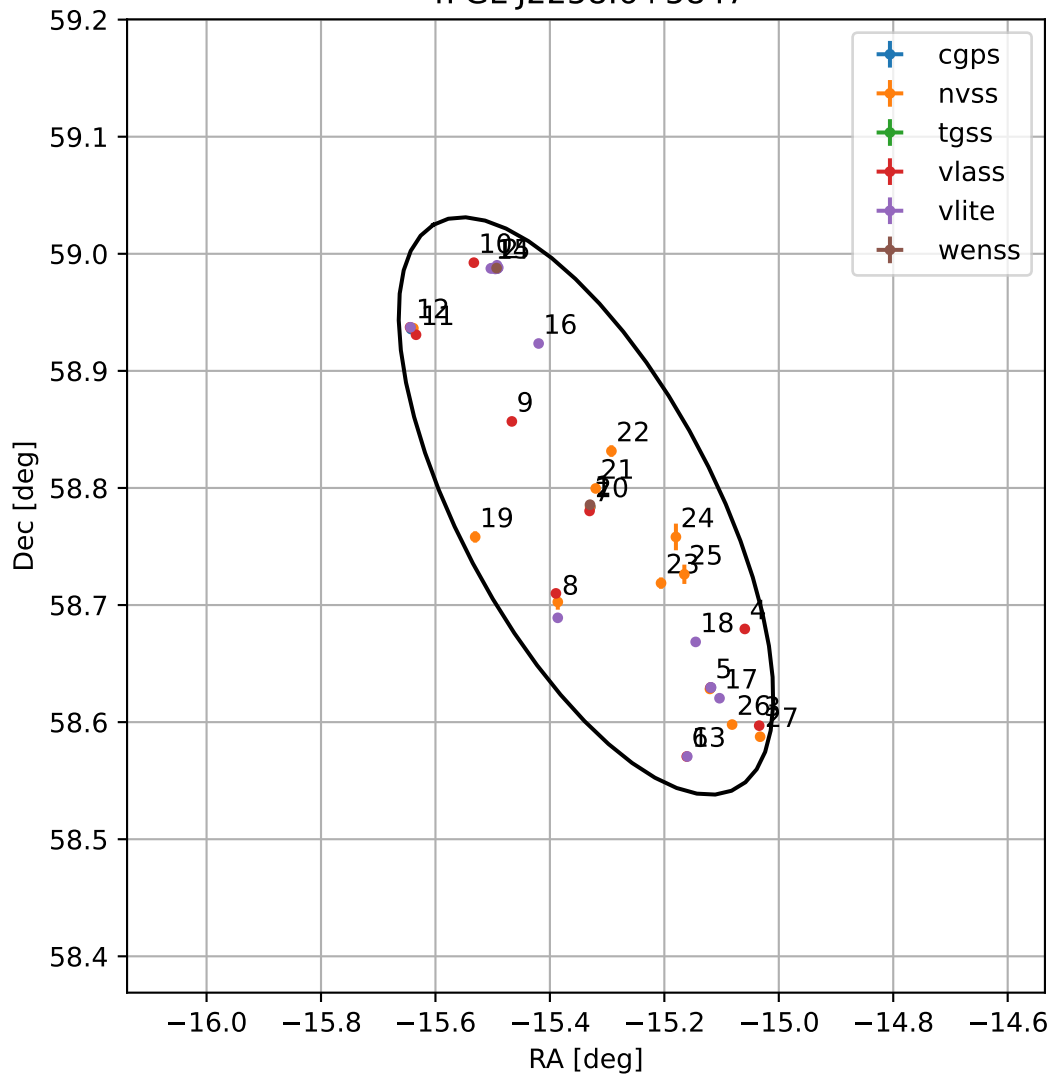
4FGL J2258.6+5847
