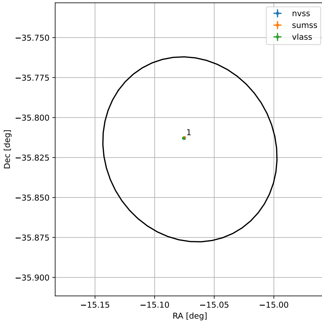
4FGL J2259.7-3549
