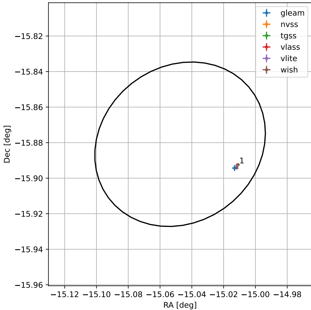
4FGL J2259.8-1552
