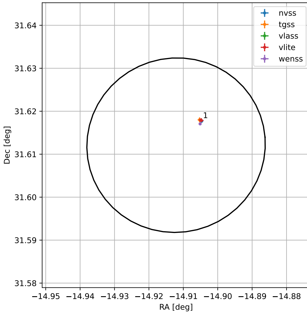
4FGL J2300.3+3136
