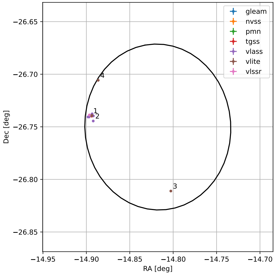
4FGL J2300.7-2645
