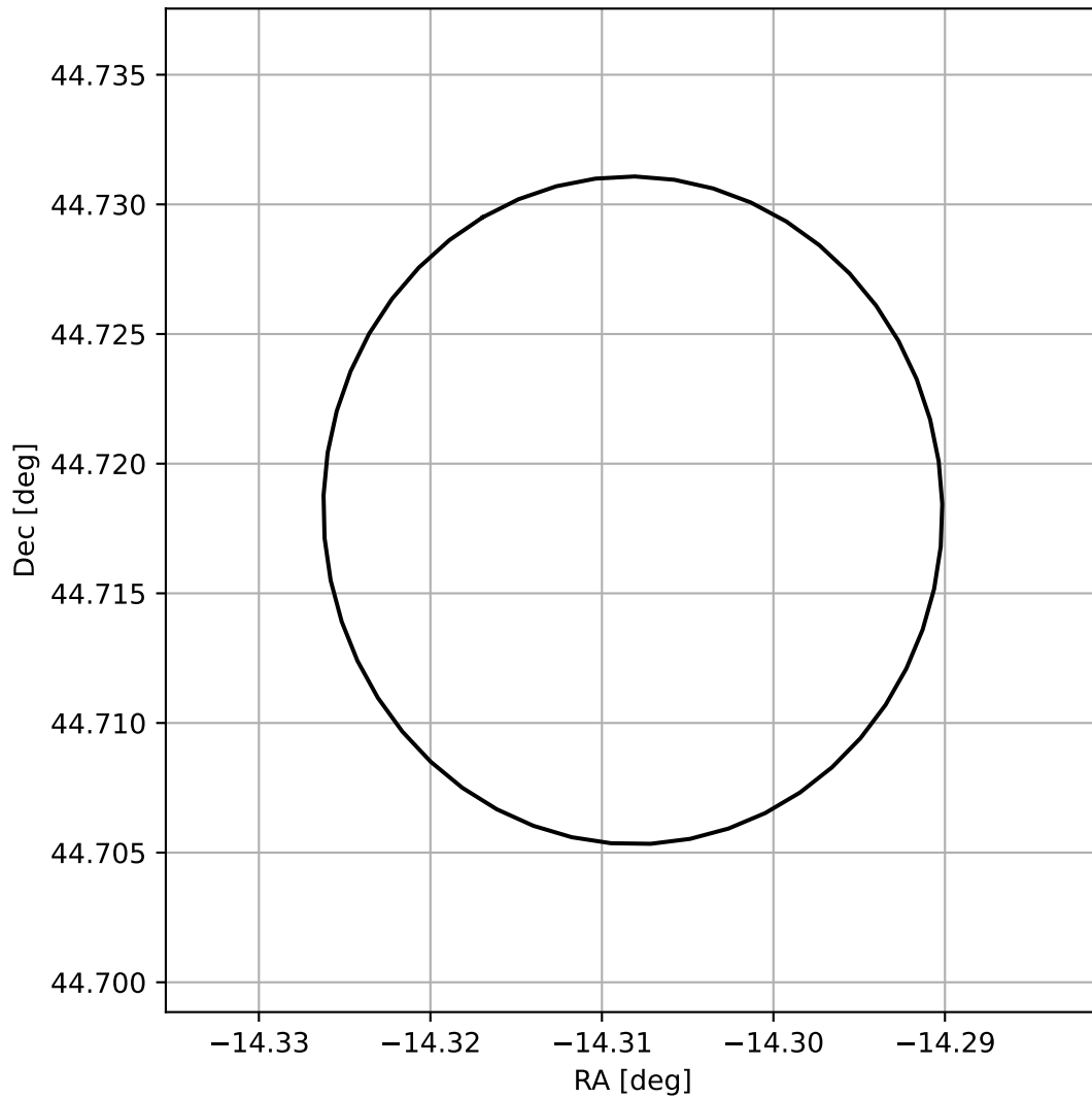
4FGL J2302.7+4443
