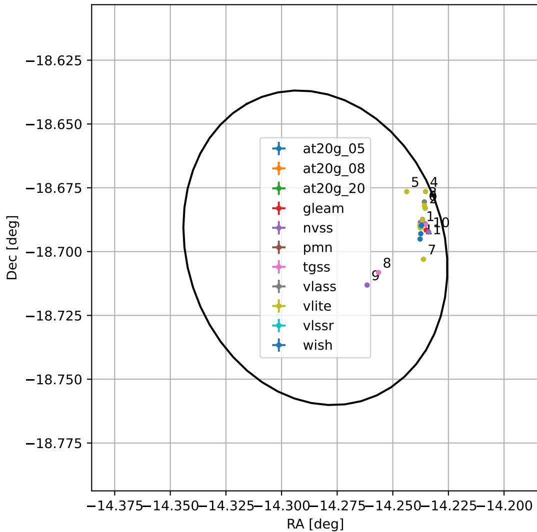
4FGL J2302.8-1841
