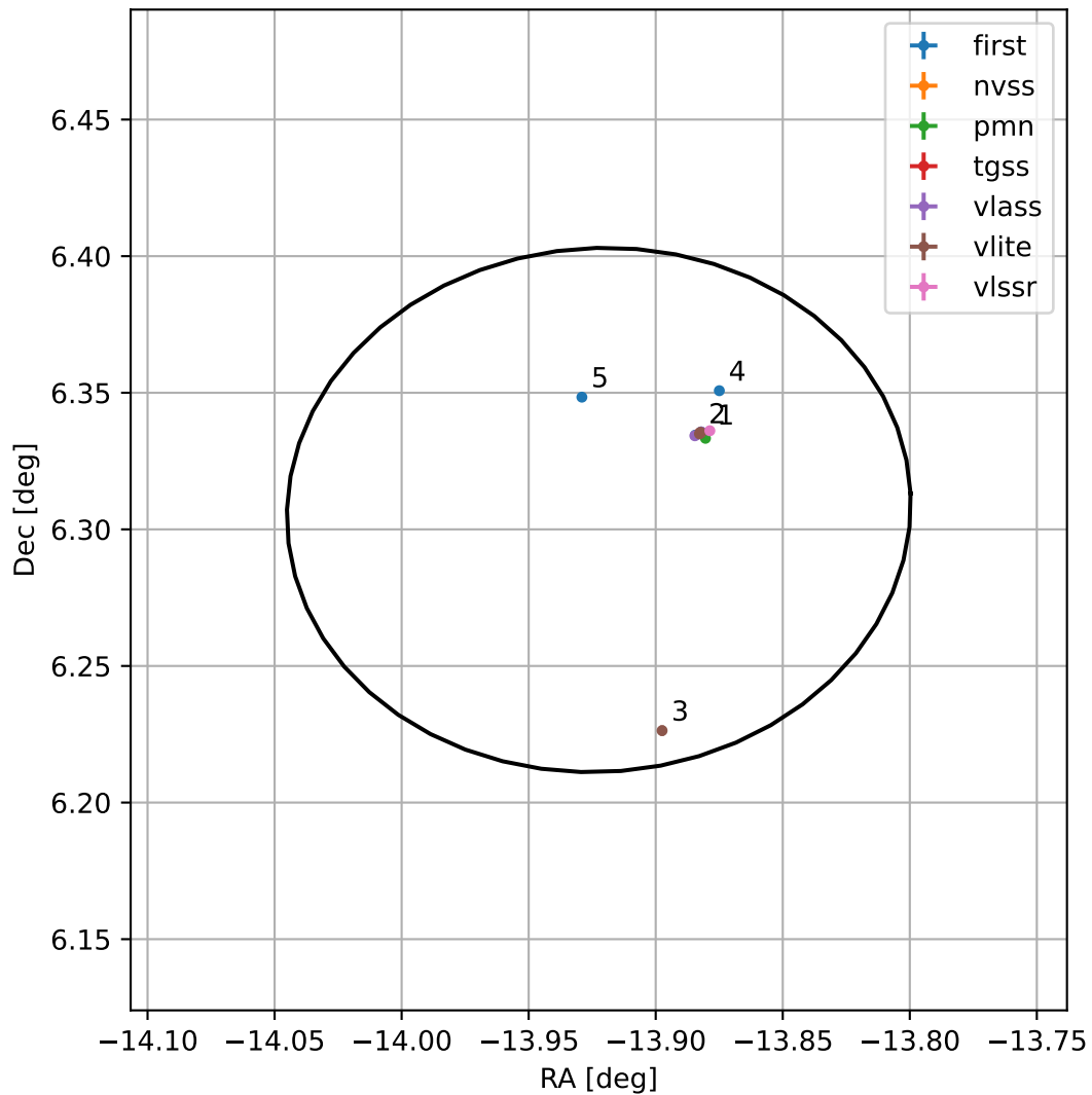
4FGL J2304.3+0618
