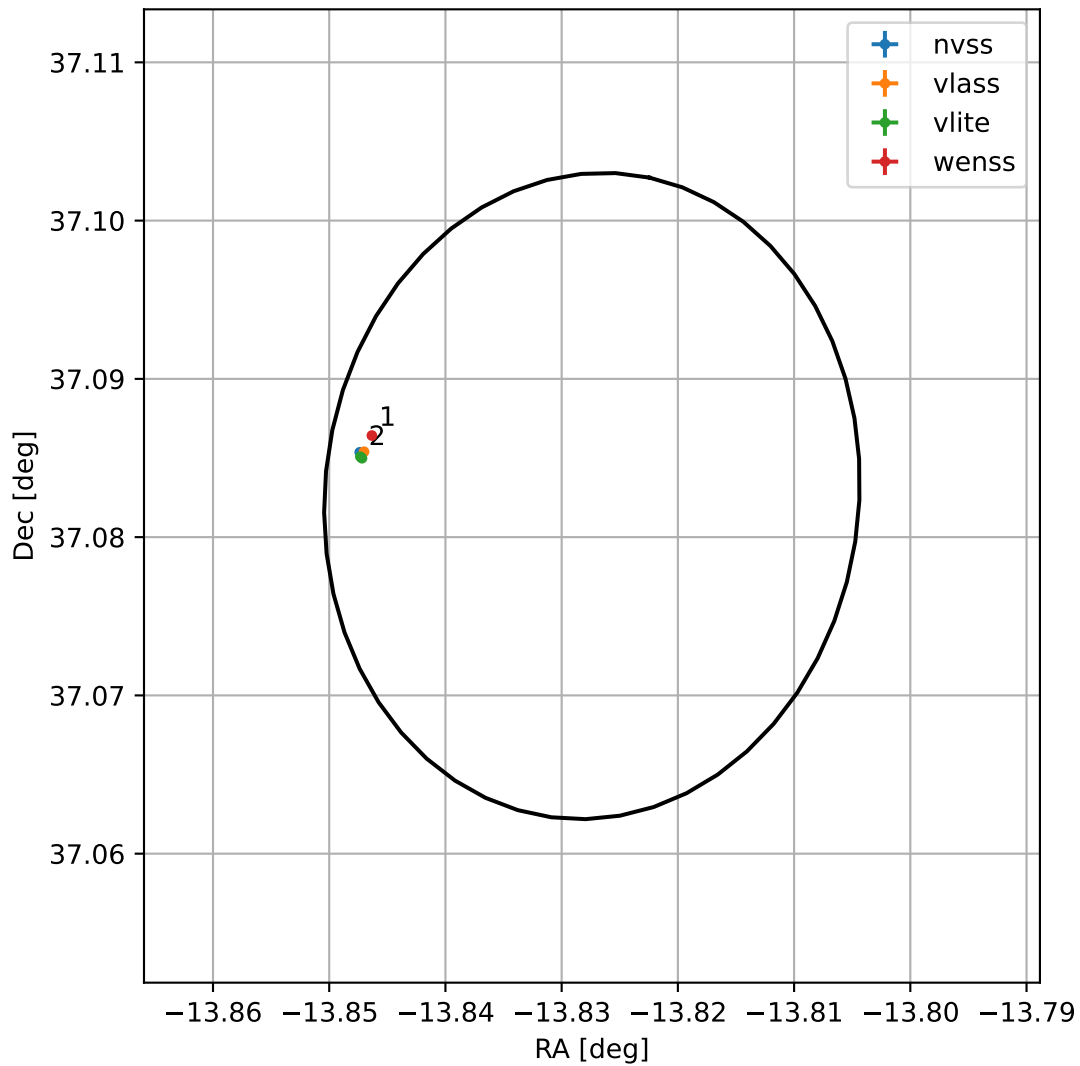
4FGL J2304.6+3704
