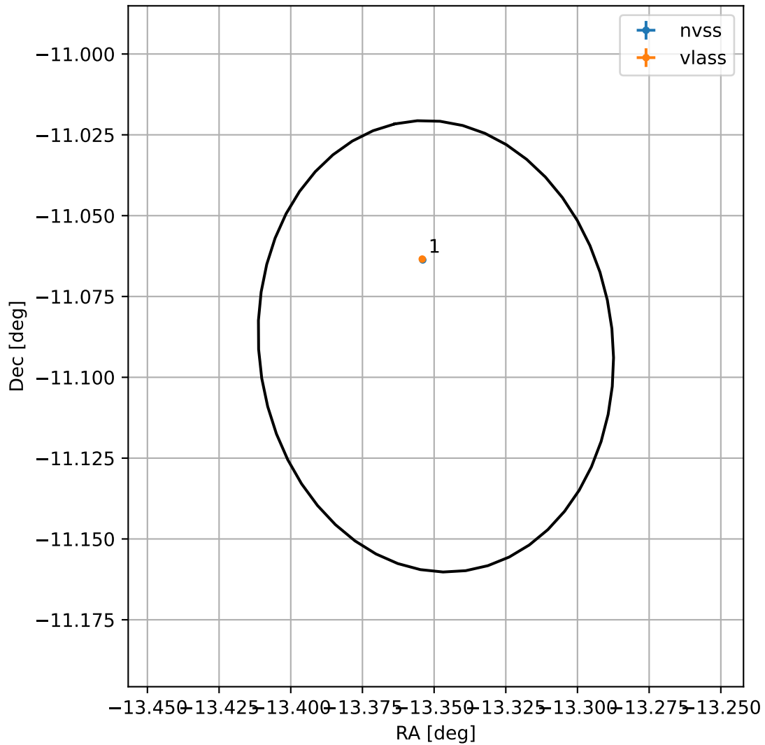
4FGL J2306.6-1105
