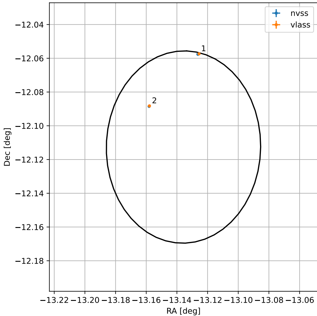
4FGL J2307.4-1206
