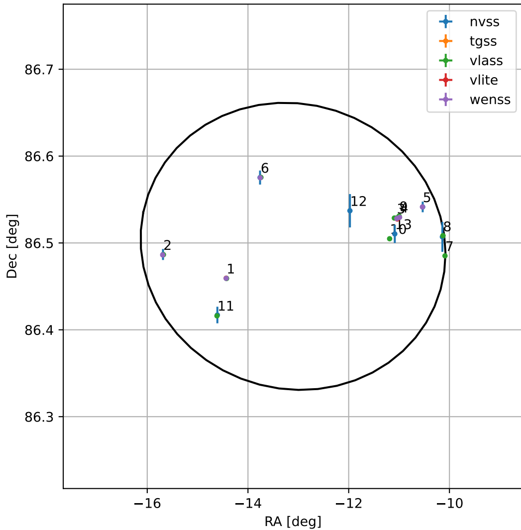
4FGL J2307.5+8629
