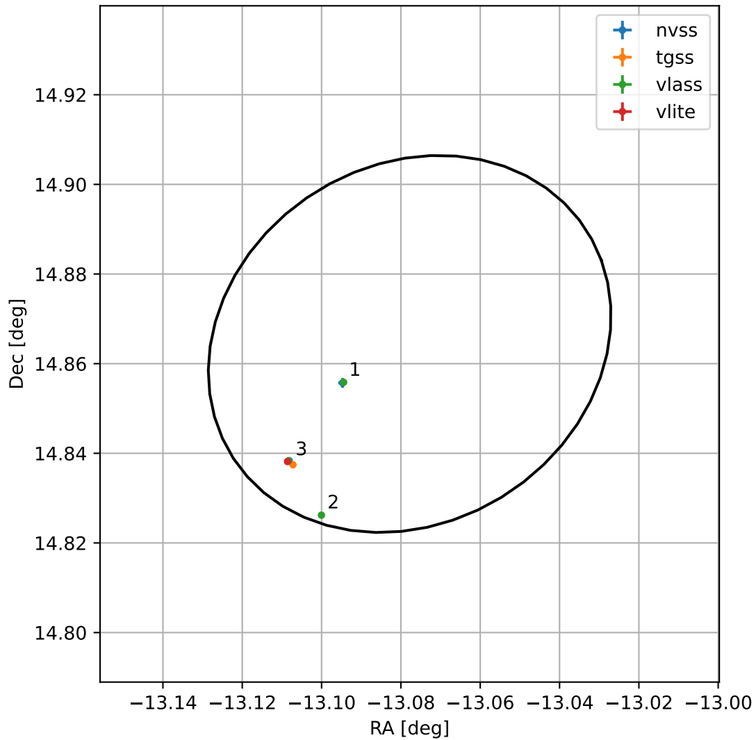
4FGL J2307.6+1451
