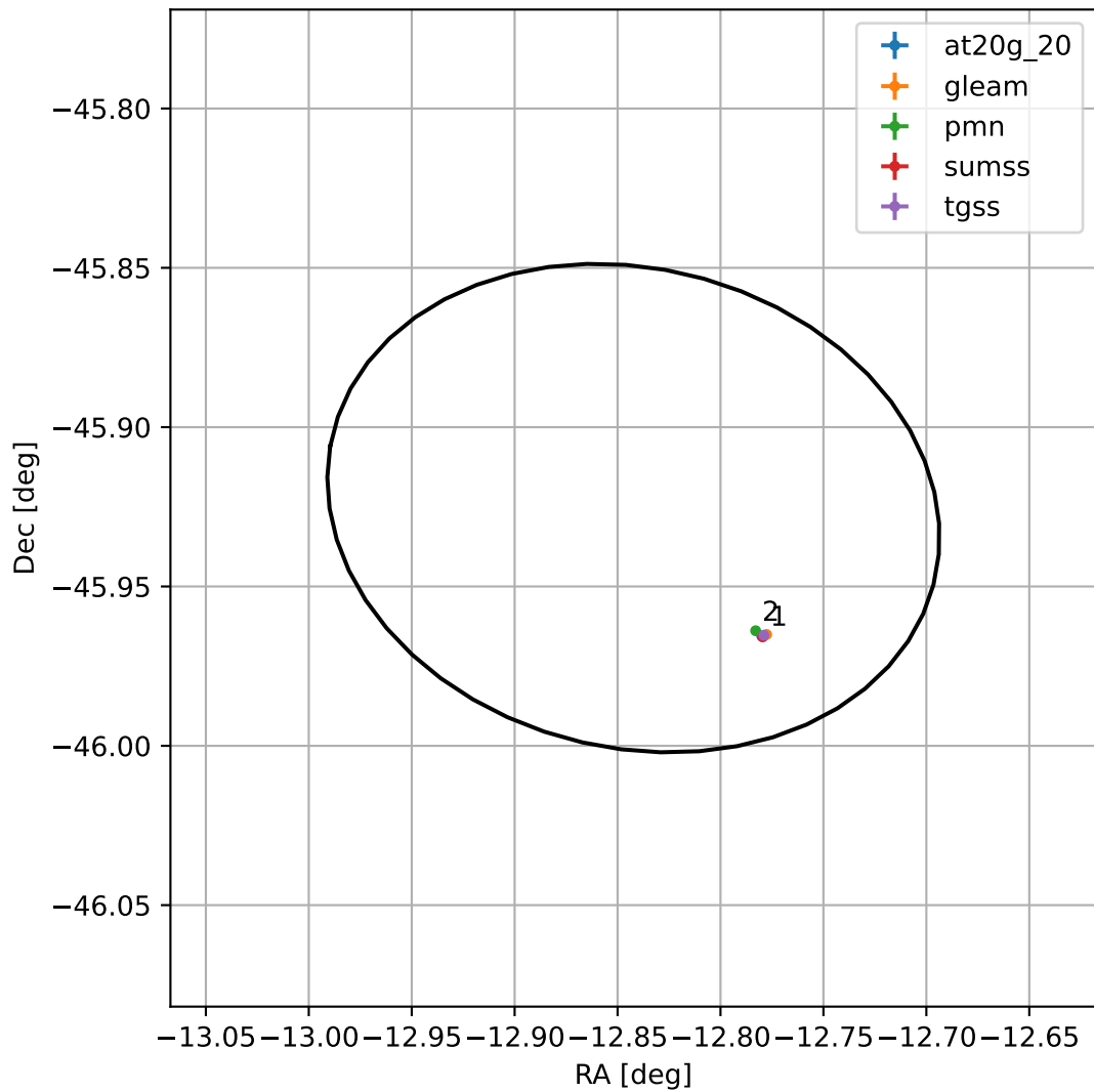
4FGL J2308.6-4555
