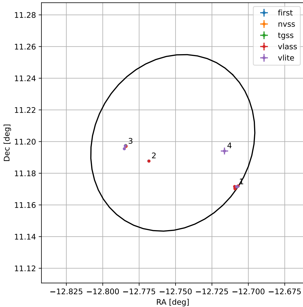
4FGL J2308.9+1111
