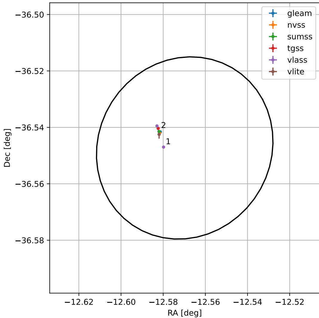
4FGL J2309.7-3632
