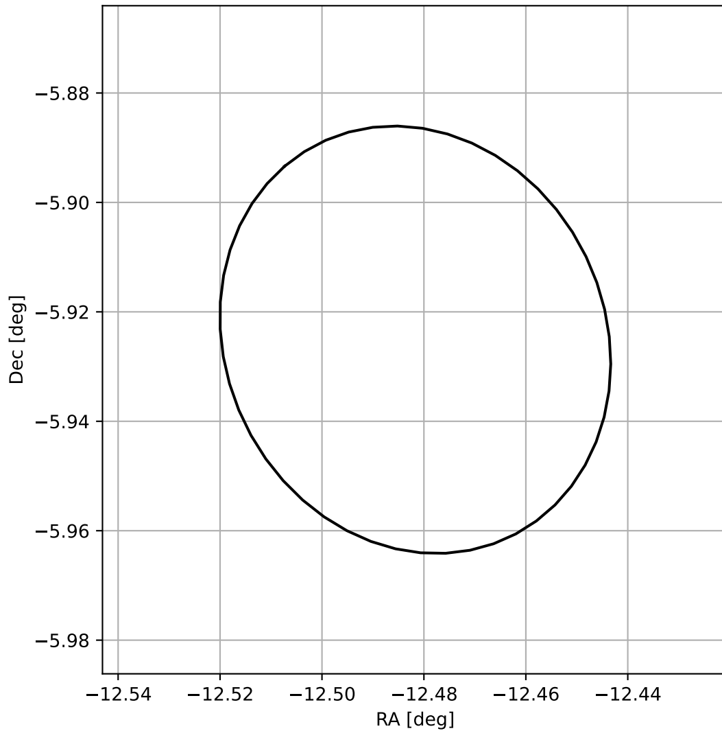
4FGL J2310.0-0555
