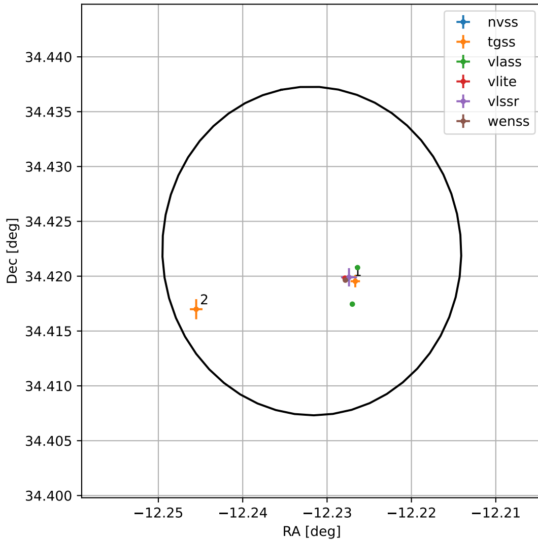
4FGL J2311.0+3425
