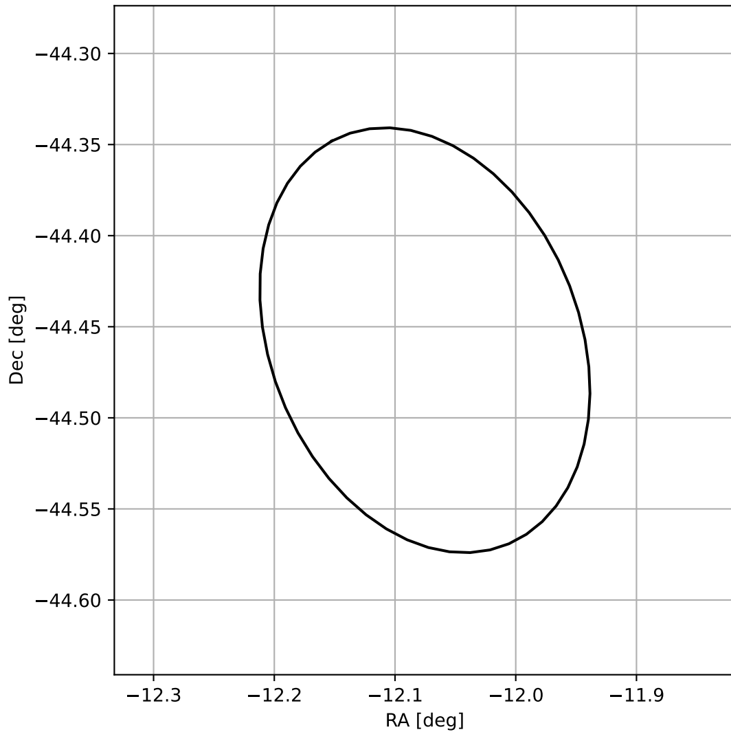
4FGL J2311.6-4427
