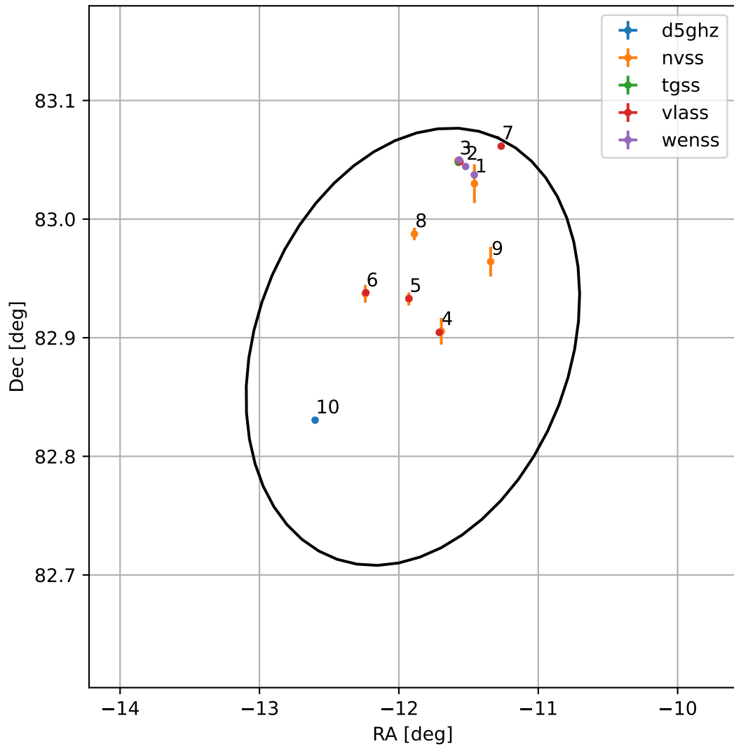
4FGL J2312.4+8253
