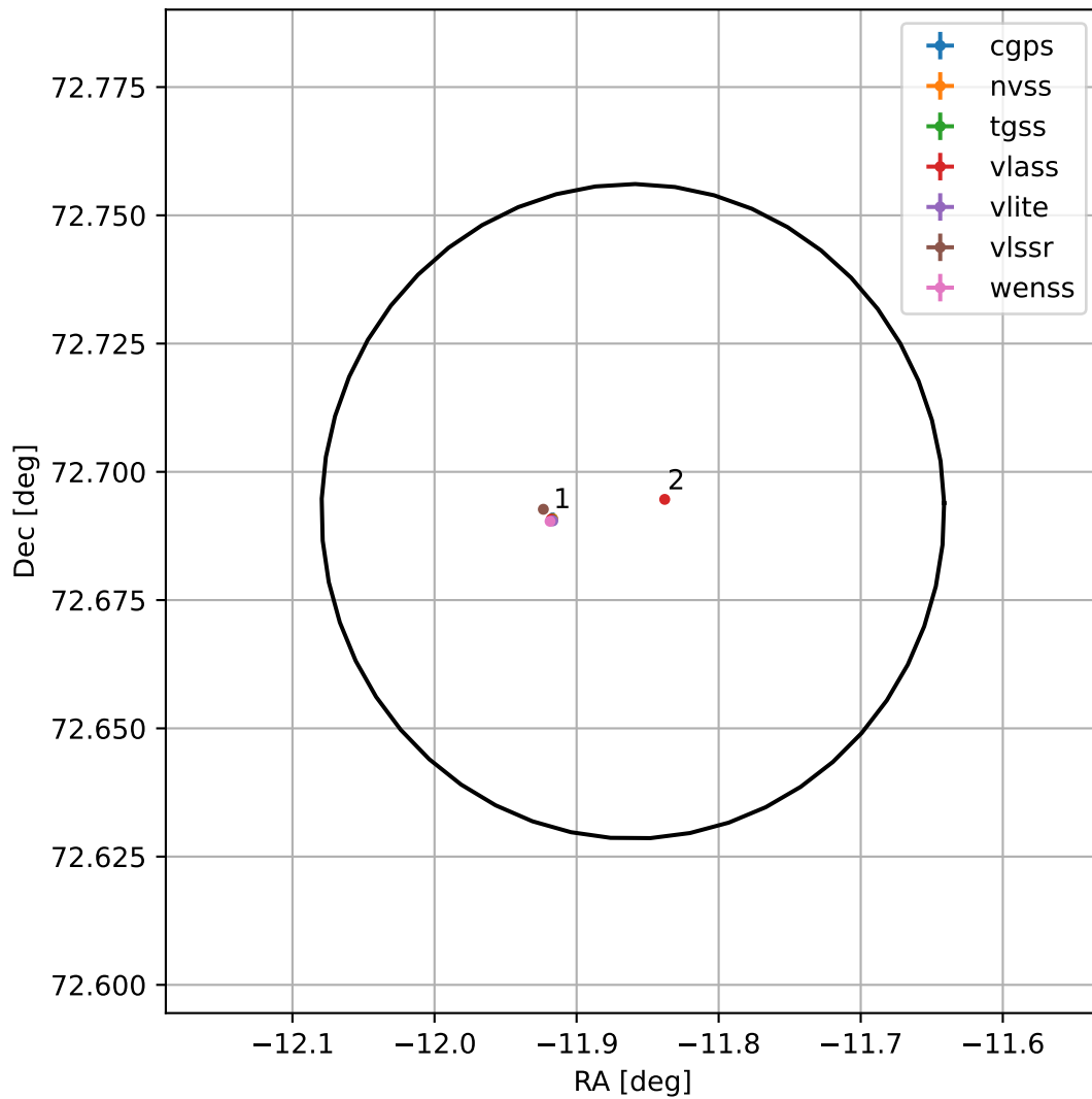
4FGL J2312.5+7241
