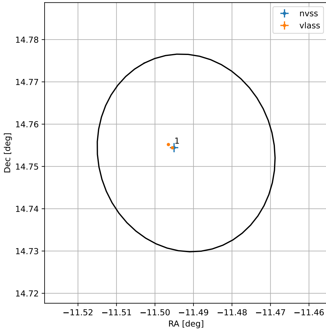
4FGL J2314.0+1445
