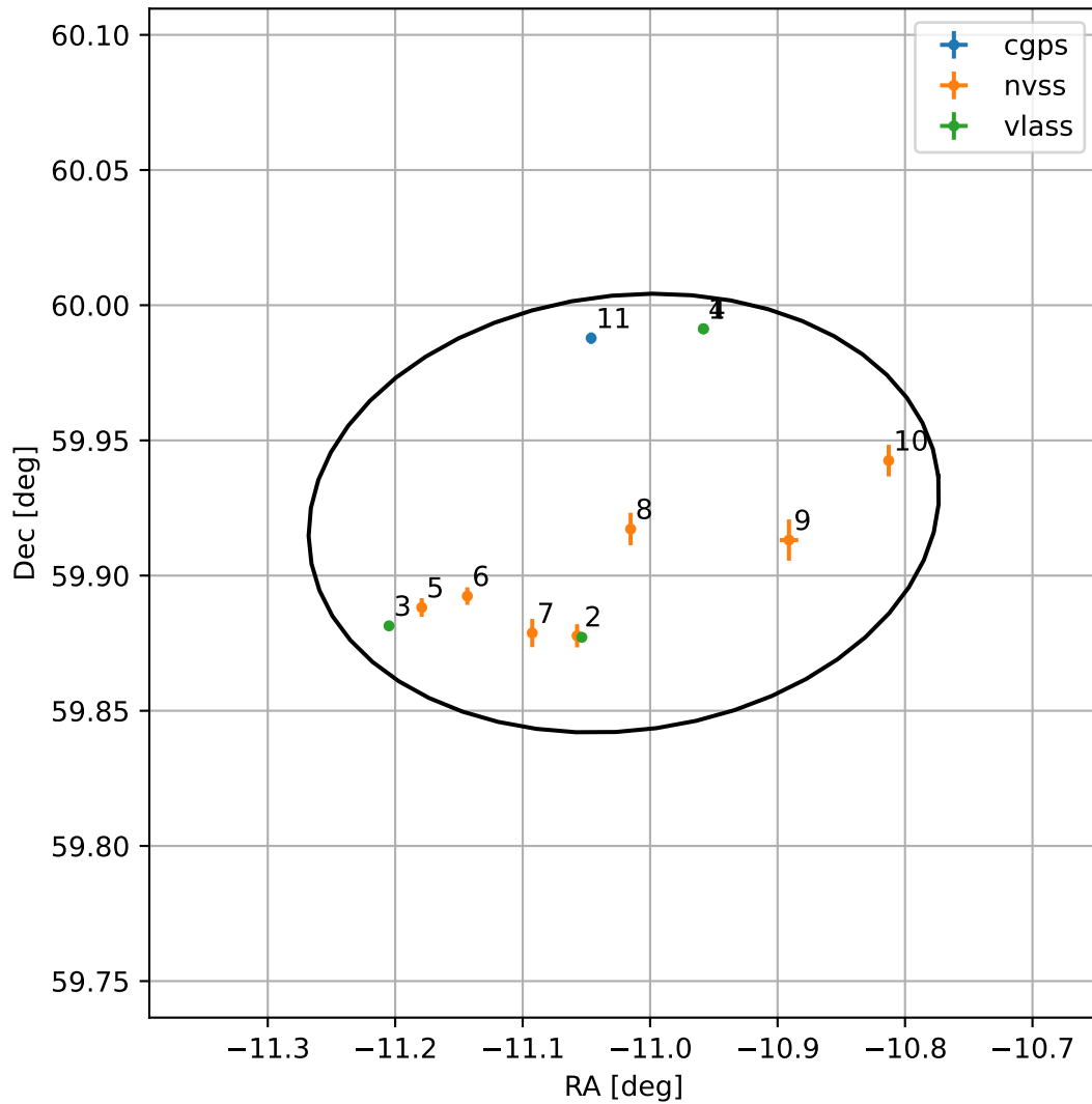
4FGL J2315.9+5955
