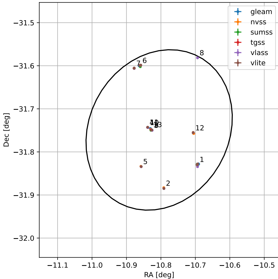
4FGL J2316.7-3144
