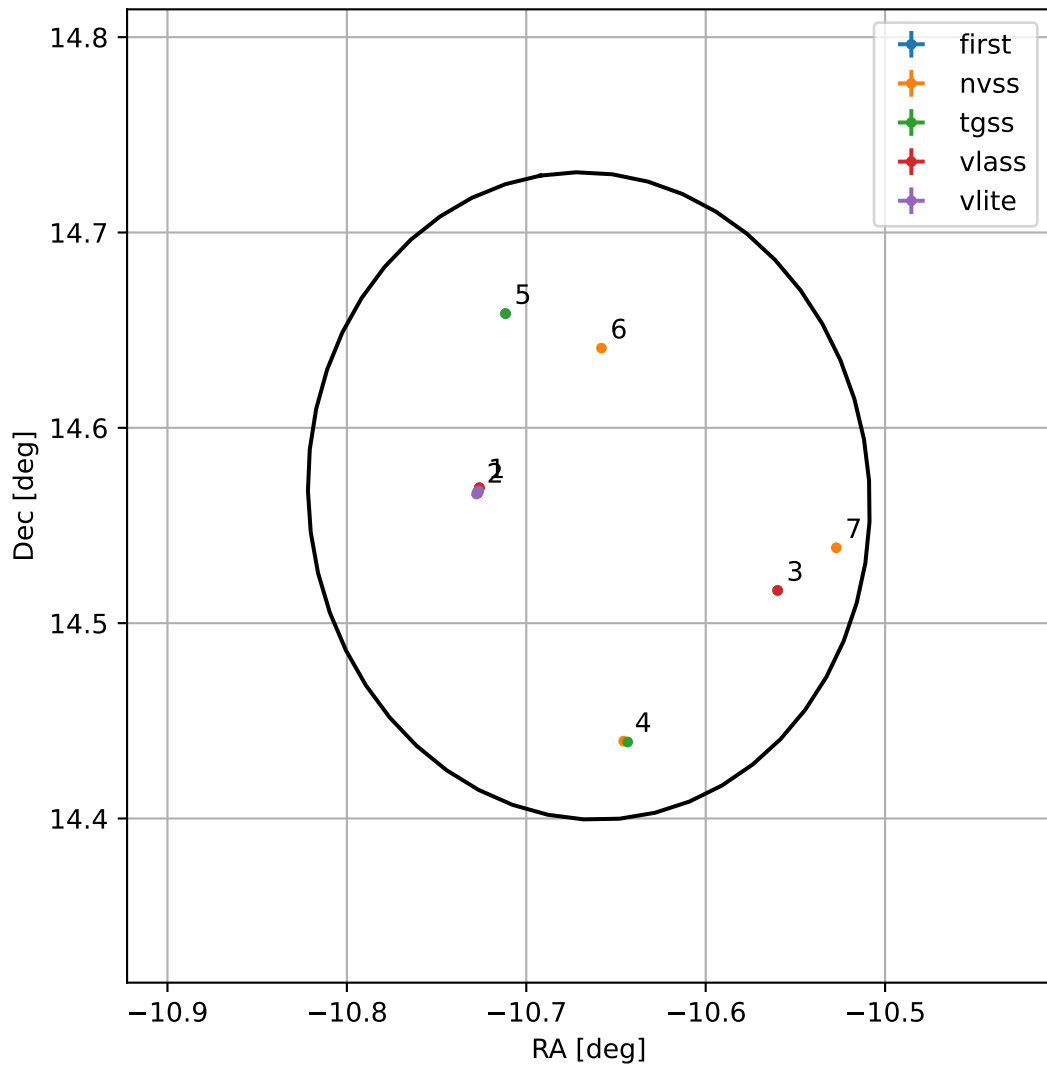
4FGL J2317.3+1433
