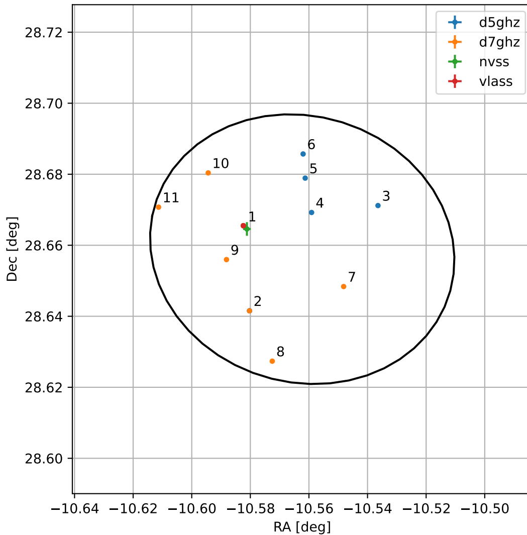
4FGL J2317.7+2839
