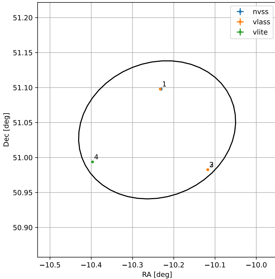
4FGL J2319.0+5102
