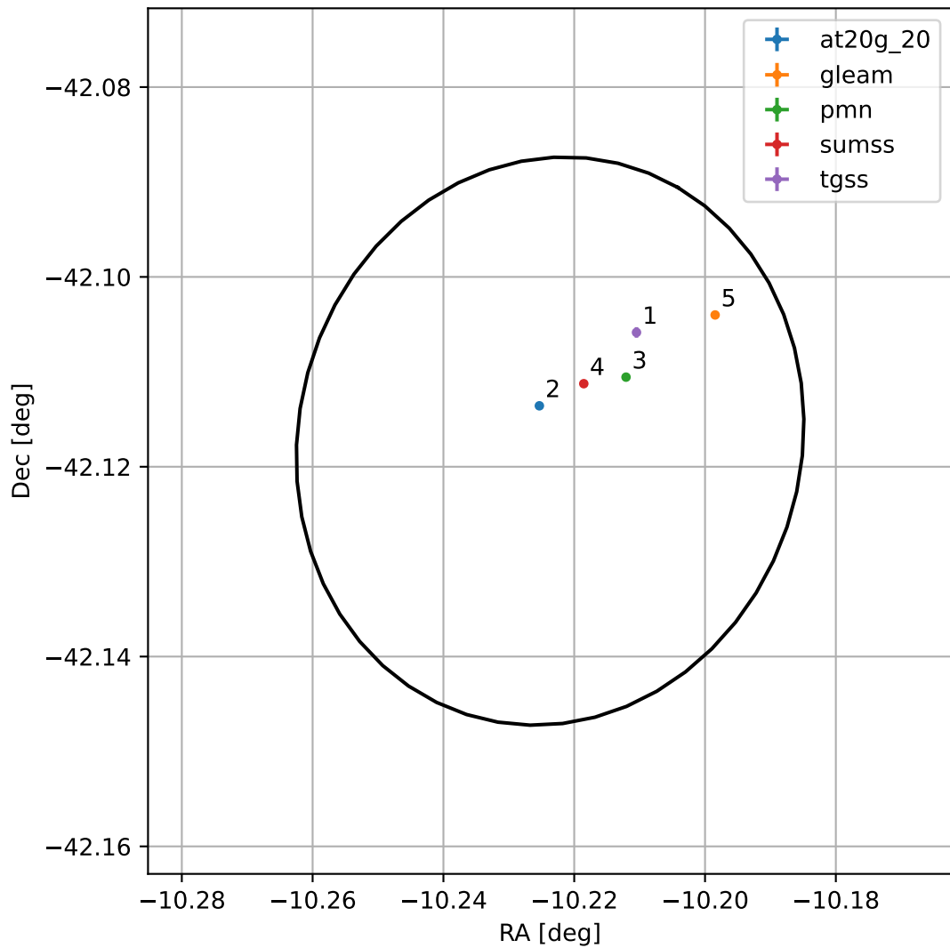
4FGL J2319.1-4207
