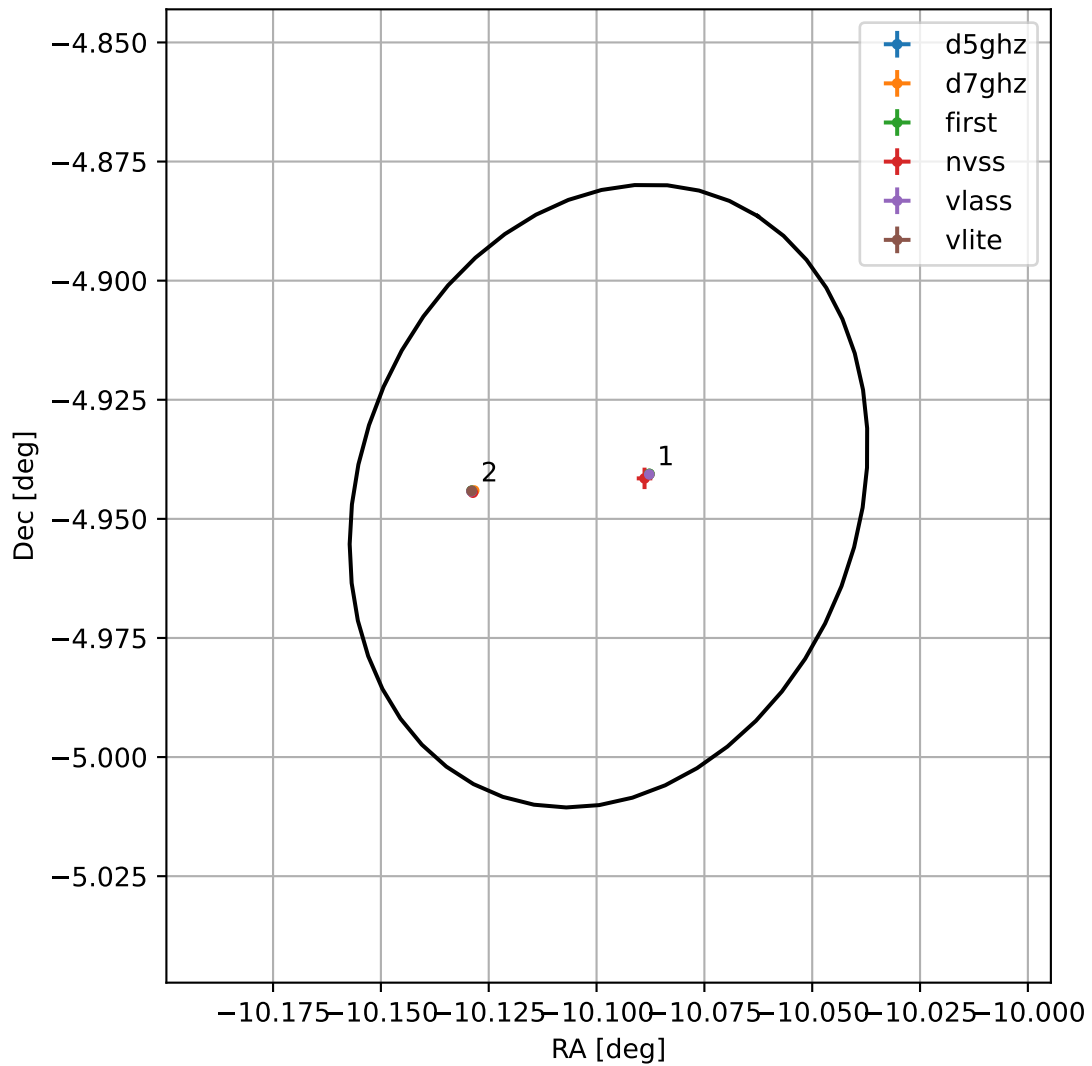
4FGL J2319.6-0456
