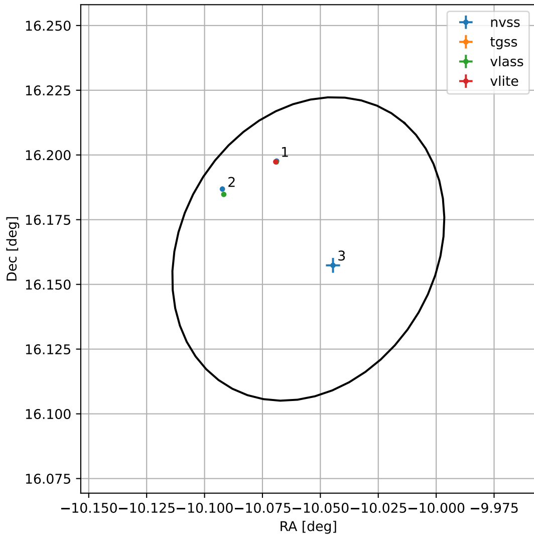
4FGL J2319.7+1609
