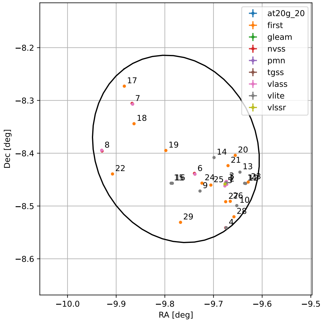
4FGL J2320.8-0823
