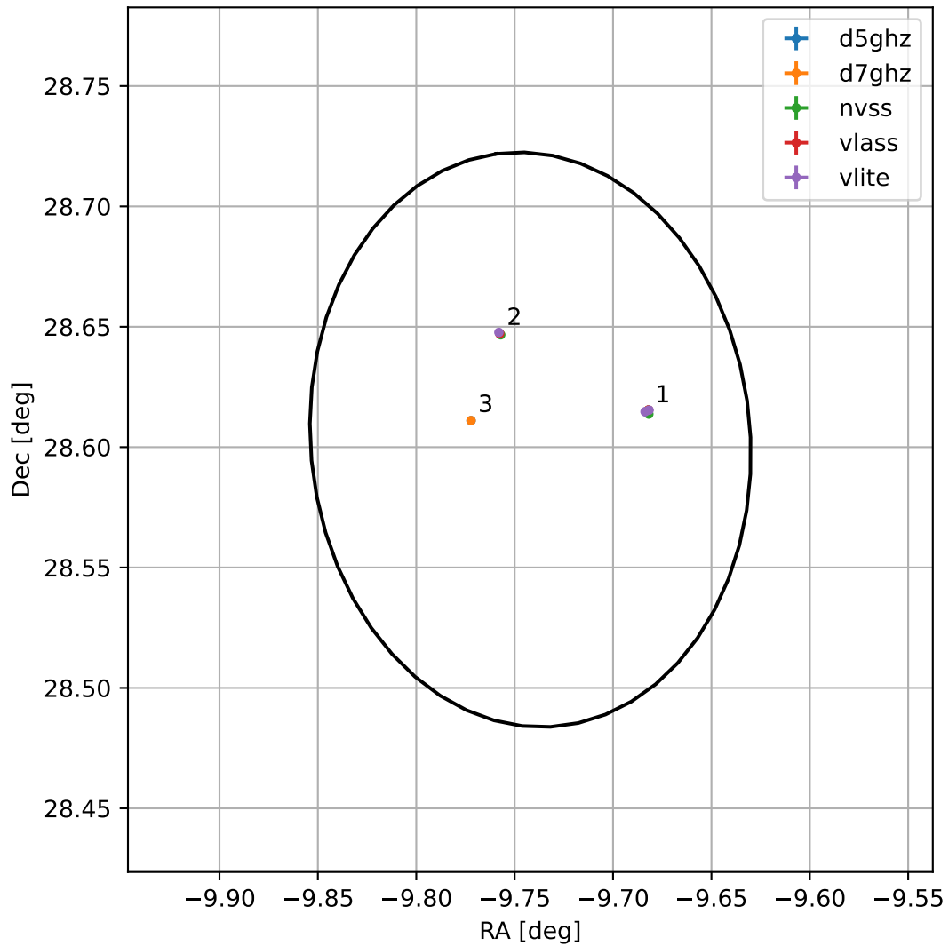
4FGL J2321.0+2836
