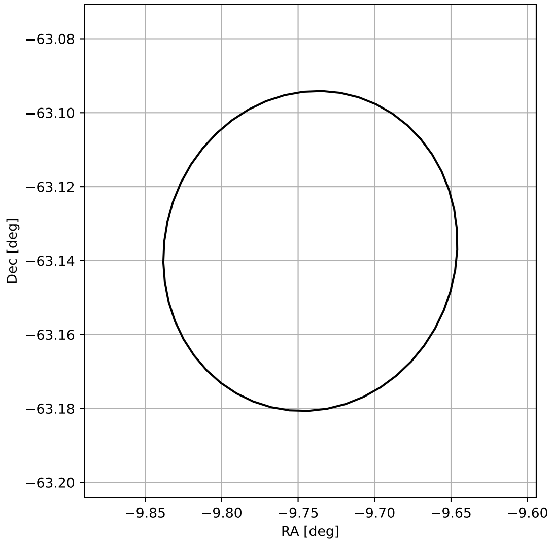
4FGL J2321.0-6308
