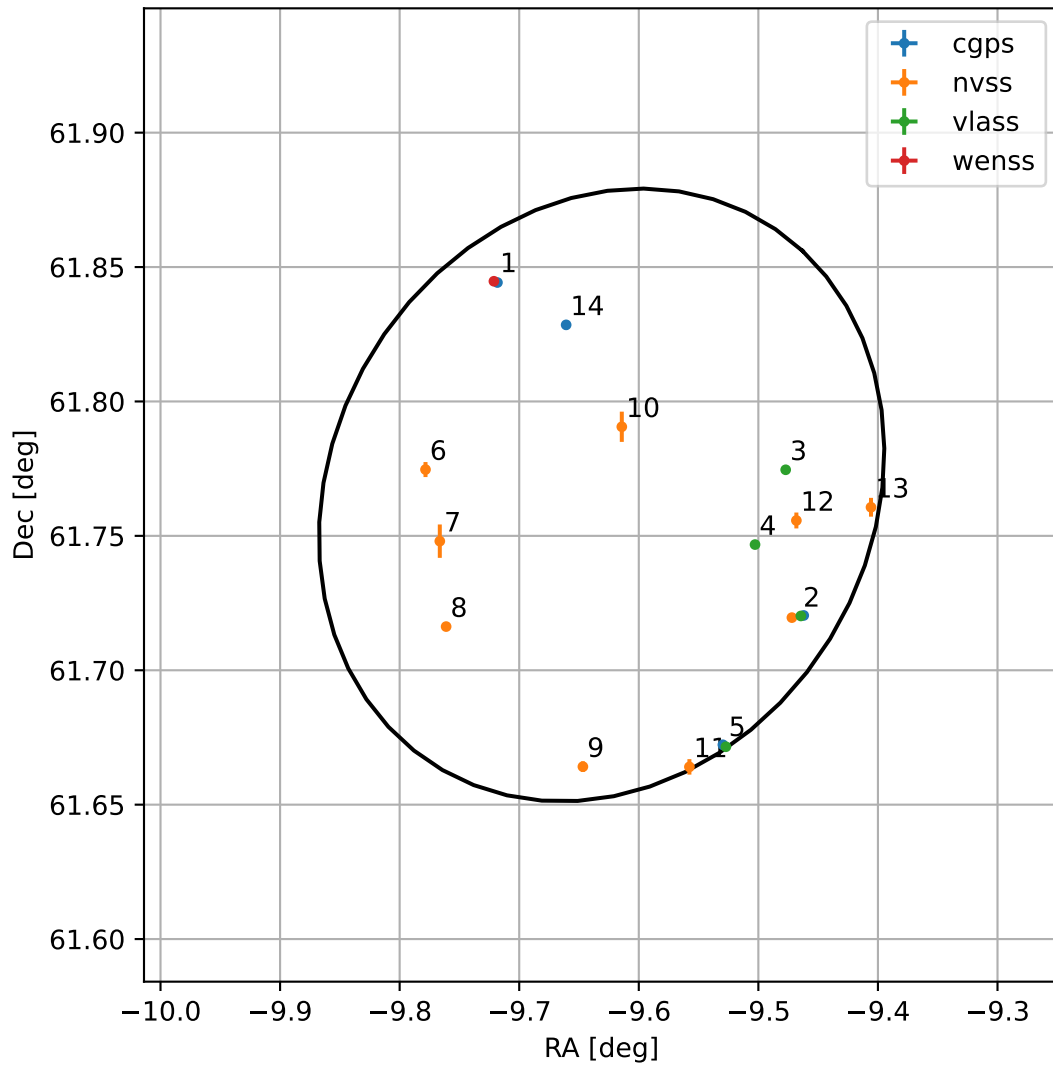
4FGL J2321.4+6145
