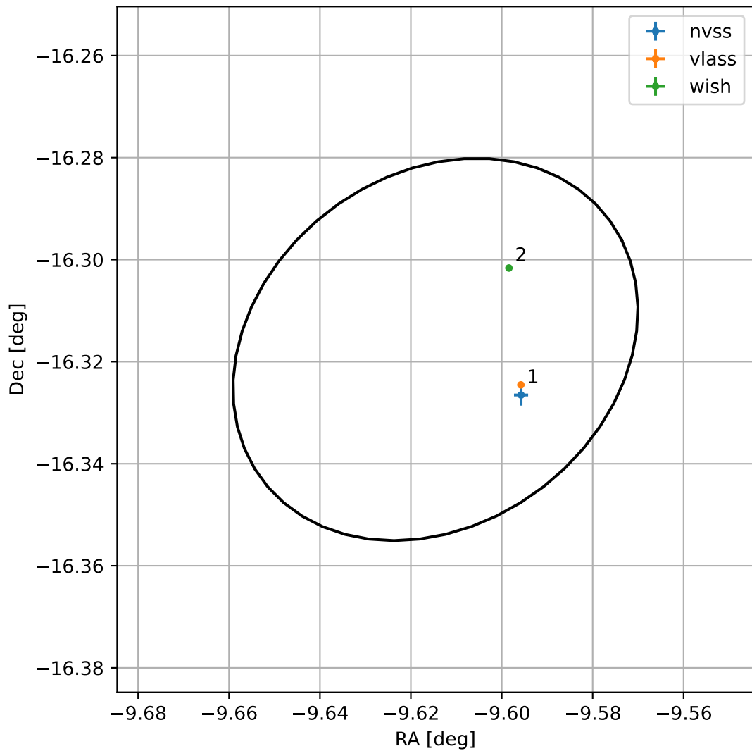
4FGL J2321.5-1619
