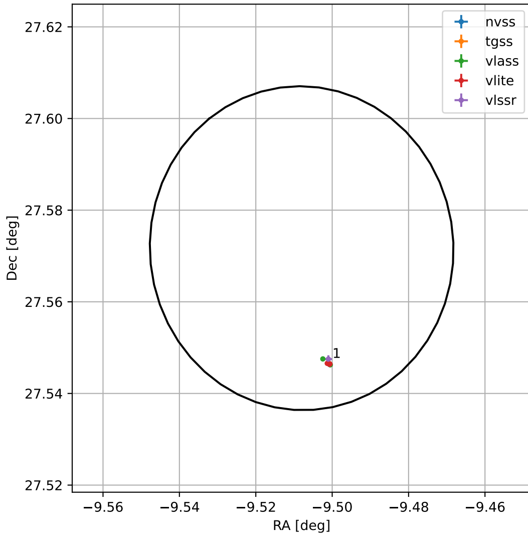
4FGL J2321.9+2734
