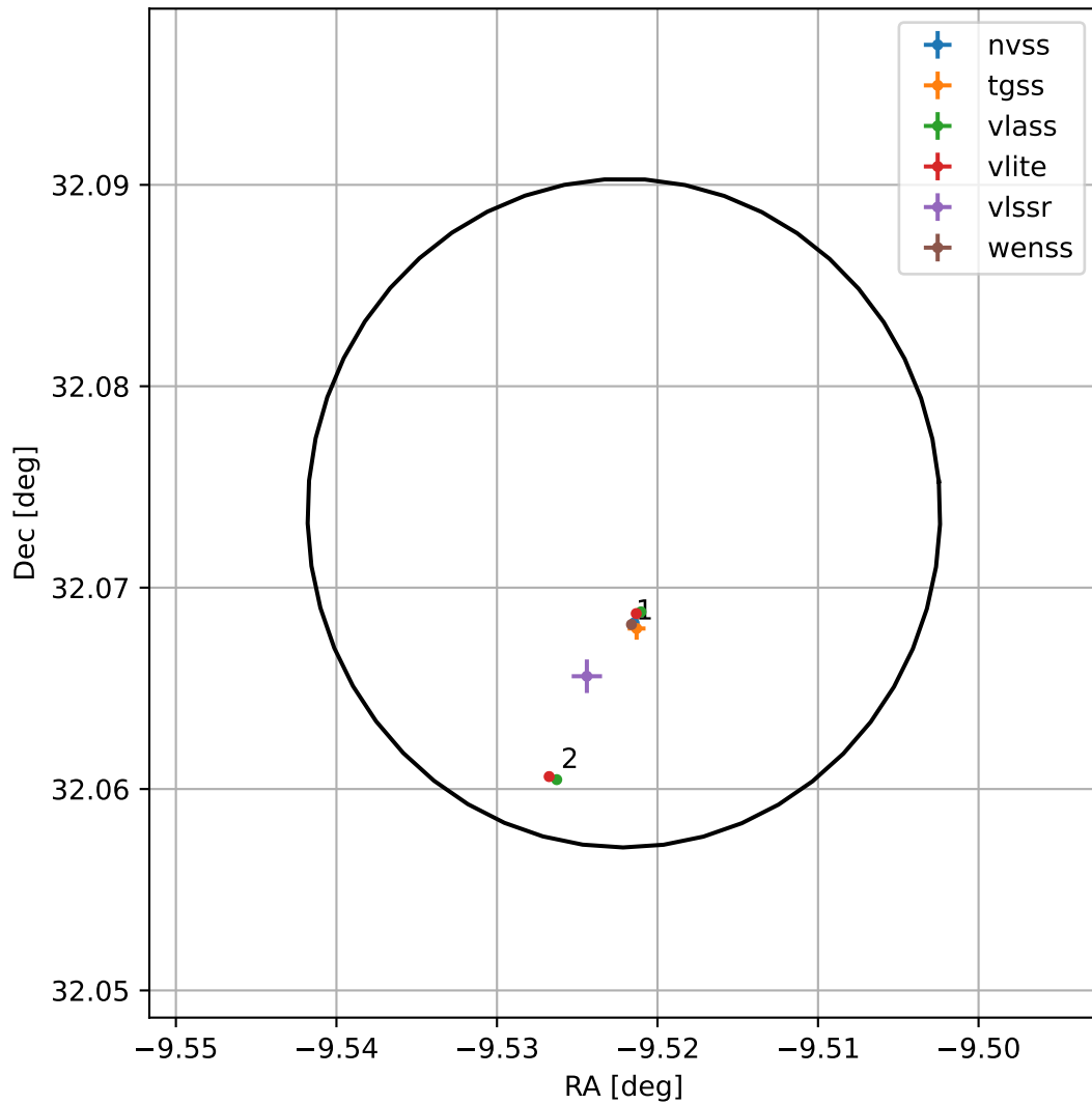
4FGL J2321.9+3204
