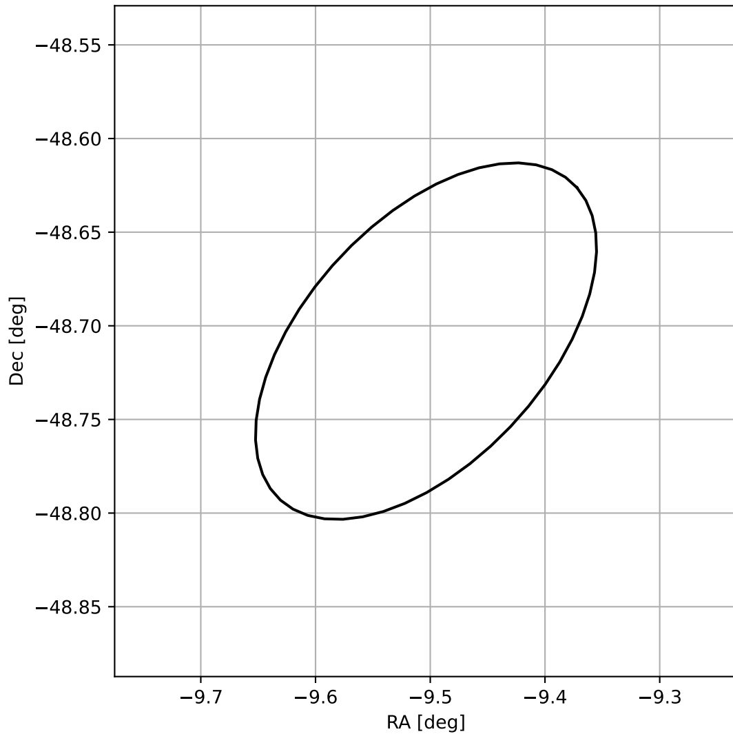
4FGL J2321.9-4842
