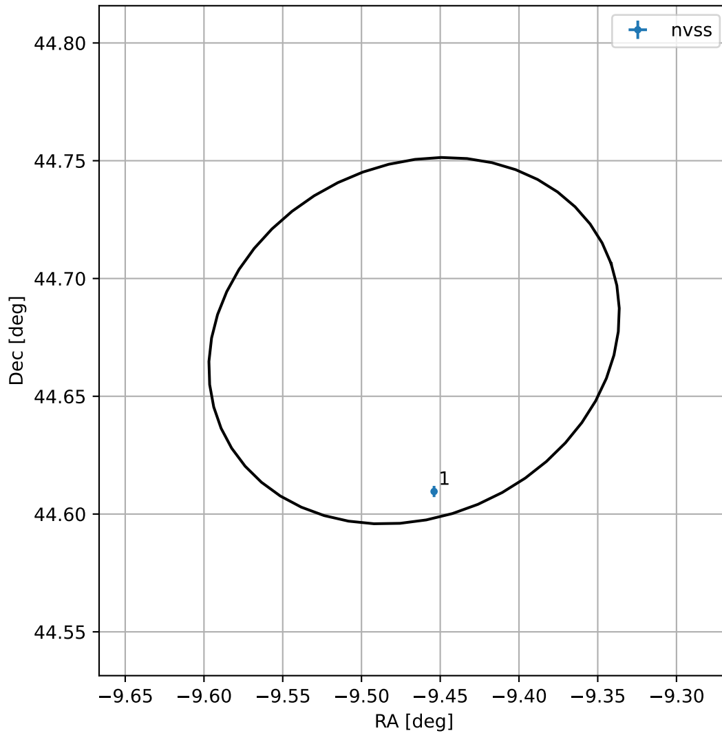
4FGL J2322.1+4440
