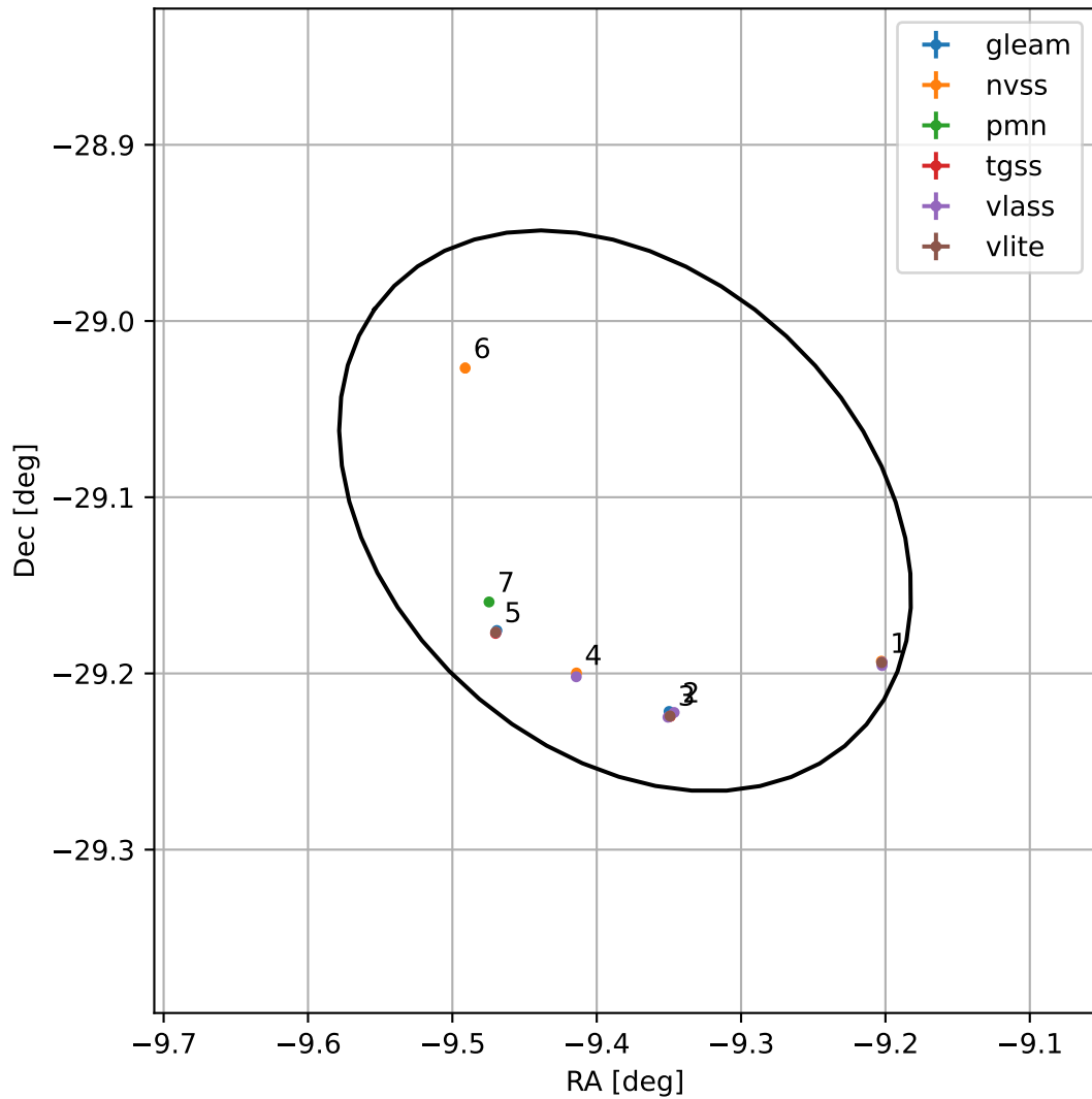
4FGL J2322.4-2906
