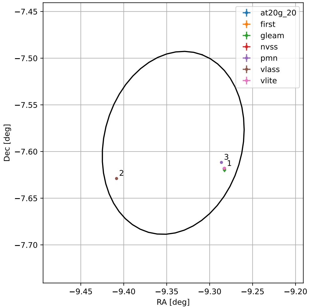
4FGL J2322.6-0735
