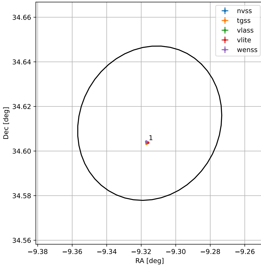
4FGL J2322.7+3436
