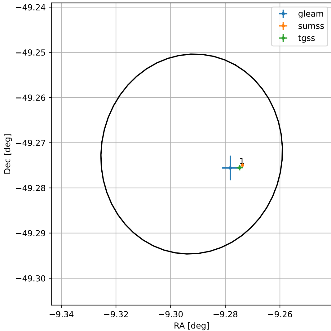
4FGL J2322.8-4916
